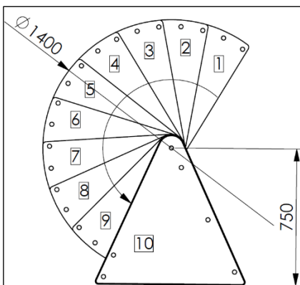
11 Stufen (Standard-1) 11 steps (standard-1)
